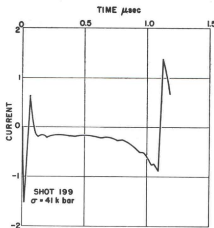
FIG. 8. 41-kbar experimental waveform.
